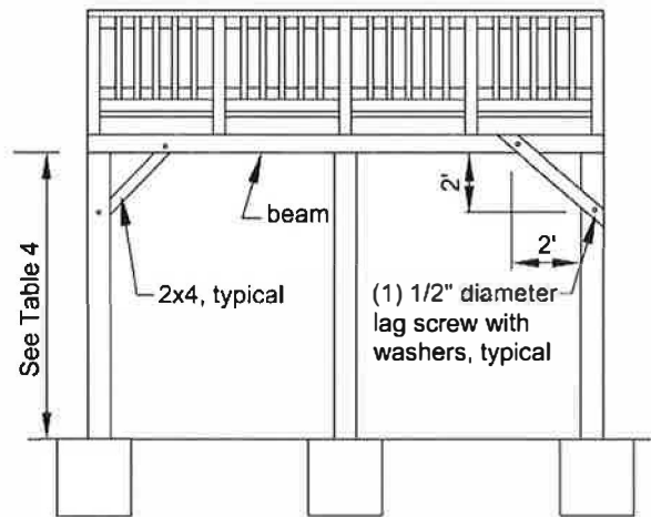
Figure 10. Diagonal Bracing.
